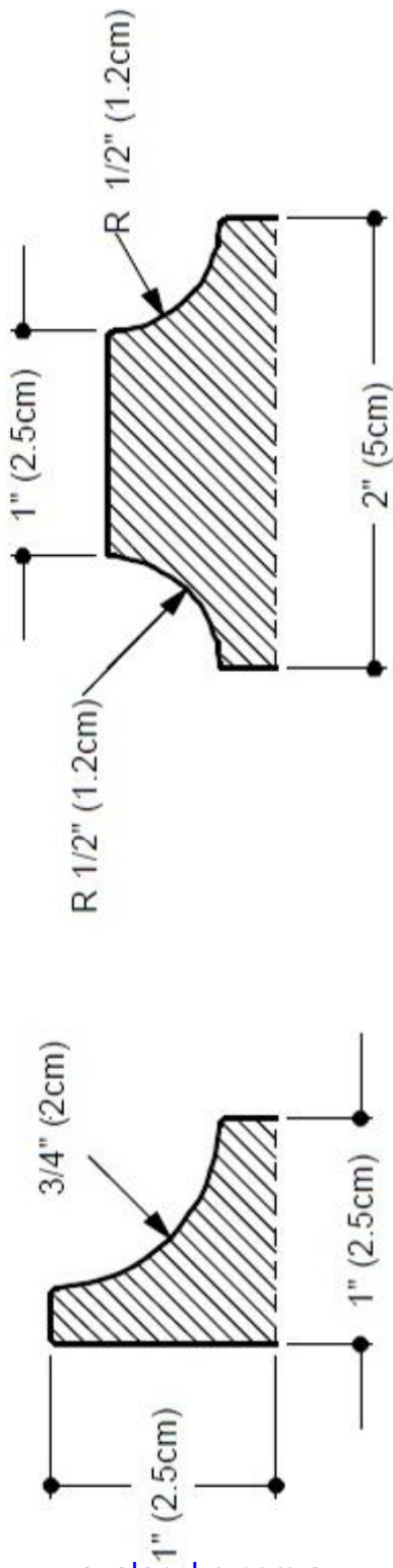
CORNER TRIM
